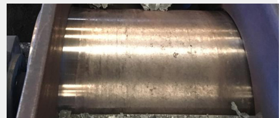
The picture shows the roller after 100,000 tons: preliminary mechanical treatment with anti-wear coating with filler material by mechanized process, and Weld Clad finishing. Where working conditions do not allow the application of carbide inserts but Customers require better durability performance, we decided to modify the design of the current rollers by adding a surface treatment with weld overlays for anti-wear purposes.
